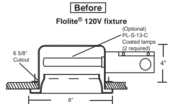
Example of 120V lighting that can be converted to our Trifecta, SoloBeam, or H-DL.
